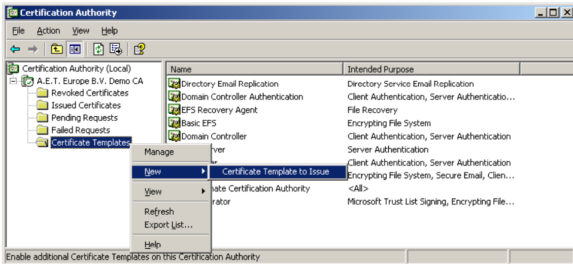
Figure 13: Certification Authority: Certificate Templates: New Certificate Template to Issue
