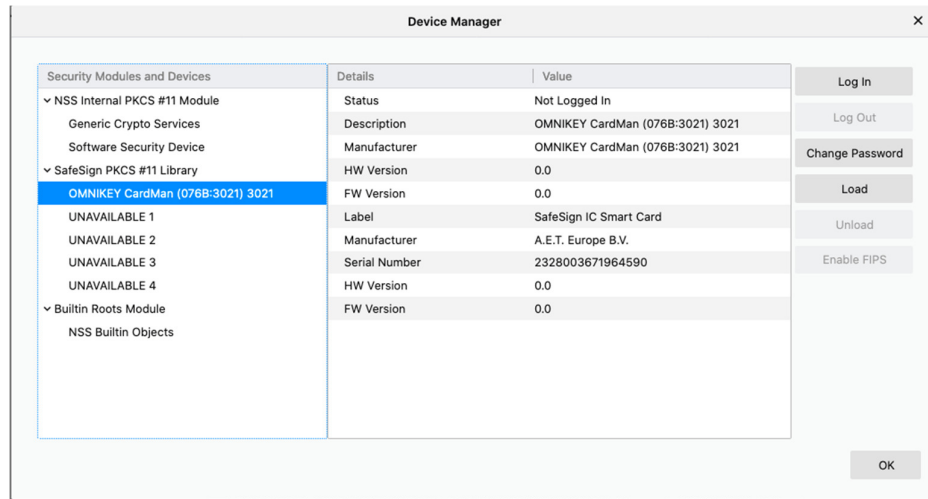
Figure 15: Firefox Device Manager: SafeSign IC Token
